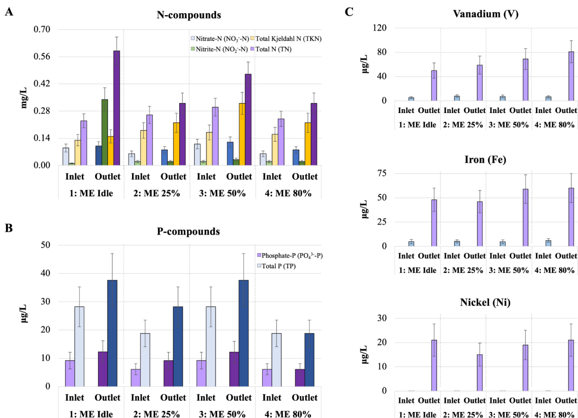
Figure 4. Nutrients and selected metals in seawater (inlet) and scrubber washwater (outlet) per engine mode. (A) N-compounds; (B) P-compounds; lighter colors indicate concentrations in incoming seawater and darker colors in washwater. (C) V, Fe, and Ni concentrations.
