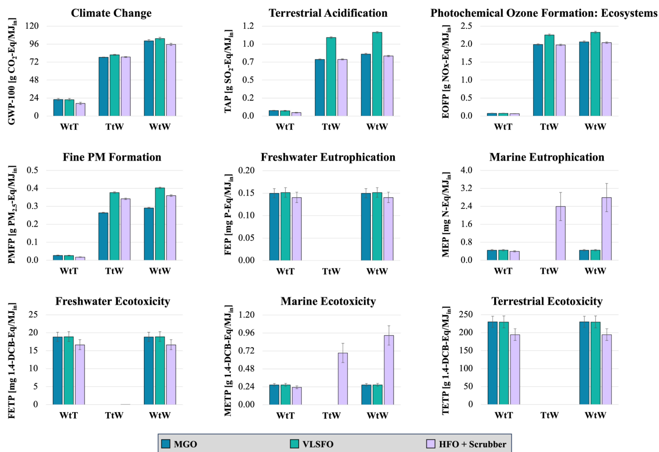
Figure 5. WtW Impacts of MGO, VLSFO and HFO combined with a scrubber per MJ of incoming energy into the vessel's engines. GWP-100: global warming potential over a 100-year time horizon; TAP: terrestrial acidification potential; EOFP: ecosystem ozone formation potential; PMFP: particulate matter formation potential; FEP: freshwater eutrophication potential; MEP: marine eutrophication potential; FETP: freshwater ecotoxicity potential; METP: marine ecotoxicity potential; TETP: terrestrial ecotoxicity potential; 1,4-DCB: 1,4-dichlorobenzene. For HFO + scrubber post-scrubber values were considered.
