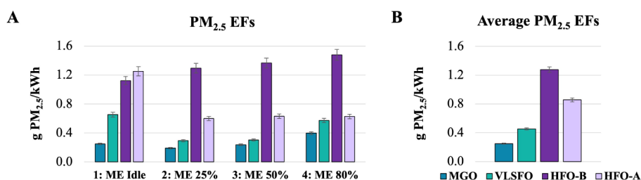
Figure 3. PM 2.5 EFs. (A) EFs per engine operating mode. (B) Vessel weighted average EFs. HFO-B and HFO-A stand for upstream (before) and downstream (after) of the scrubber, respectively.
