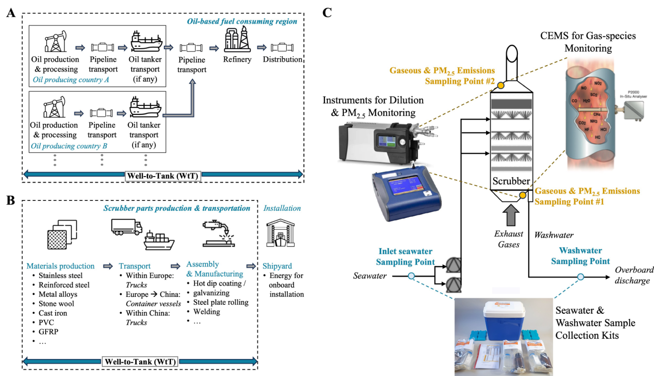
Figure 1. WtT considerations and onboard measurements. (A) The WtT system boundaries of the considered fuels, including all stages from oil extraction up to fuel bunkering aboard the vessel. (B) The WtT system boundaries of the scrubber, including all stages from raw materials production up to the installation of the scrubber aboard the vessel at the shipyard; the shipyard stage is not included in the analysis. (C) Schematic diagram of the onboard emission monitoring systems. (Images adapted or sourced from refs. 38–43 )
