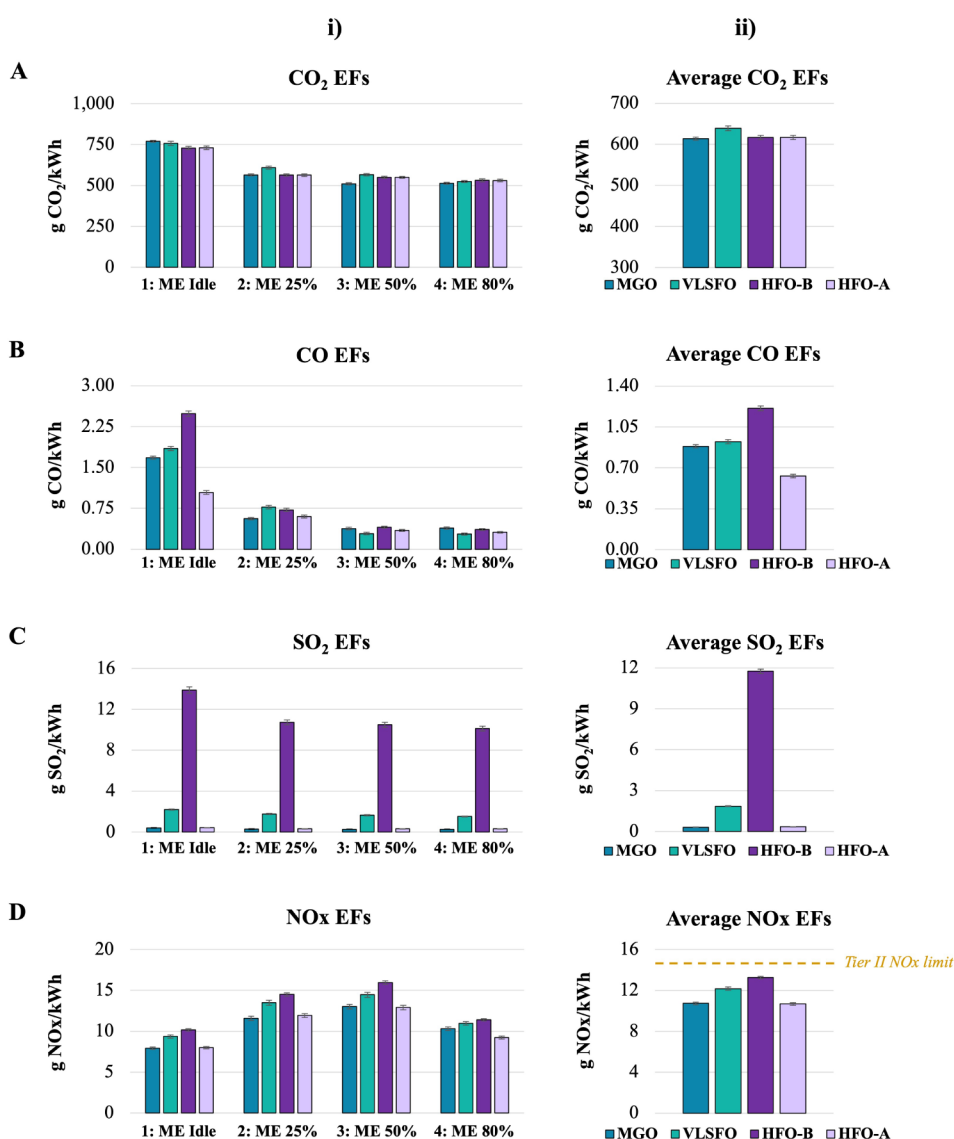
Figure 2. Gas EFs. Columns are ordered as follows: EFs per engine operating mode (i), vessel weighted average EFs (ii). (A) CO 2 EFs. (B) CO EFs. (C) SO 2 EFs. (D) NO x EFs; the orange dotted line represents the Tier II NO x emissions limit for bulk carriers operating with engine speed <130 rpm, i.e., 14.4 g kW -1 h -1 . HFO-B and HFO-A stand for upstream (before) and downstream (after) of the scrubber, respectively.
